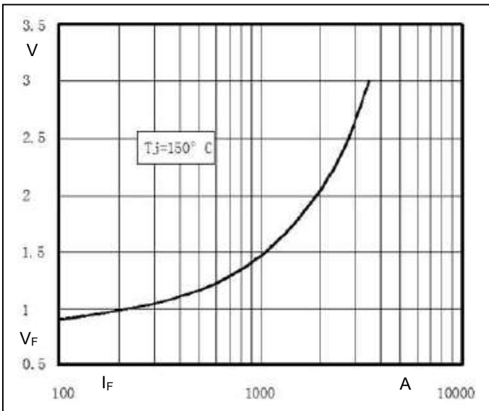
Fig1. Forward Characteristics
